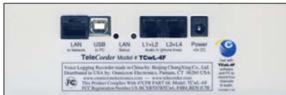
Back with input and output connections
